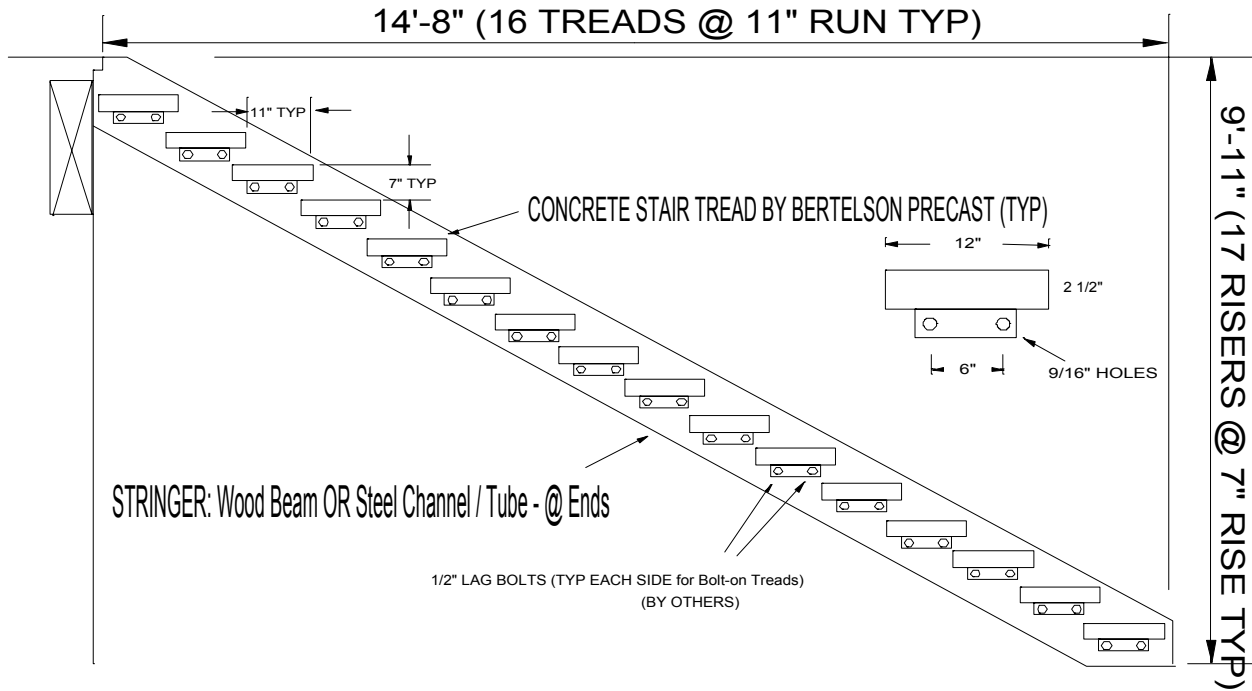
SECTION VIEW
