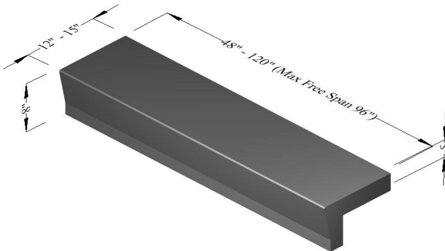
Wide Span Closed Riser Tread - Straight Nose Profile
