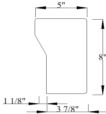
Wide Span Closure Piece - Bevel Nose Profile
