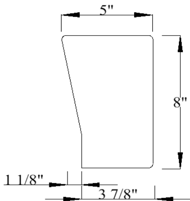
Wide Span Closure Piece - Straight Nose Profile
