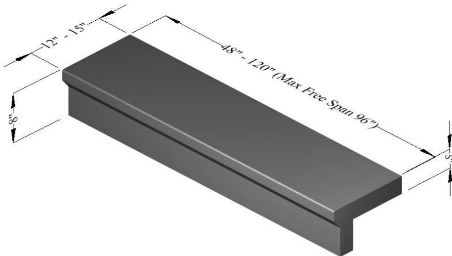
Wide Span Closed Riser Tread - Bevel Nose Profile
